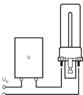
SINGLE LAMP WITH CONTROL GEAR
